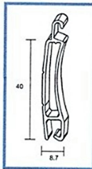
Slat Profile
